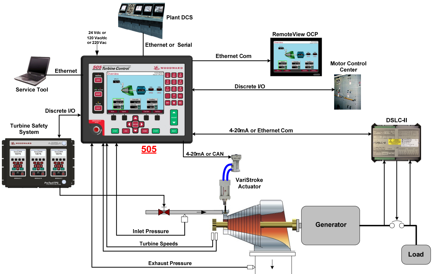
Figure 3. Typical 505 Application
