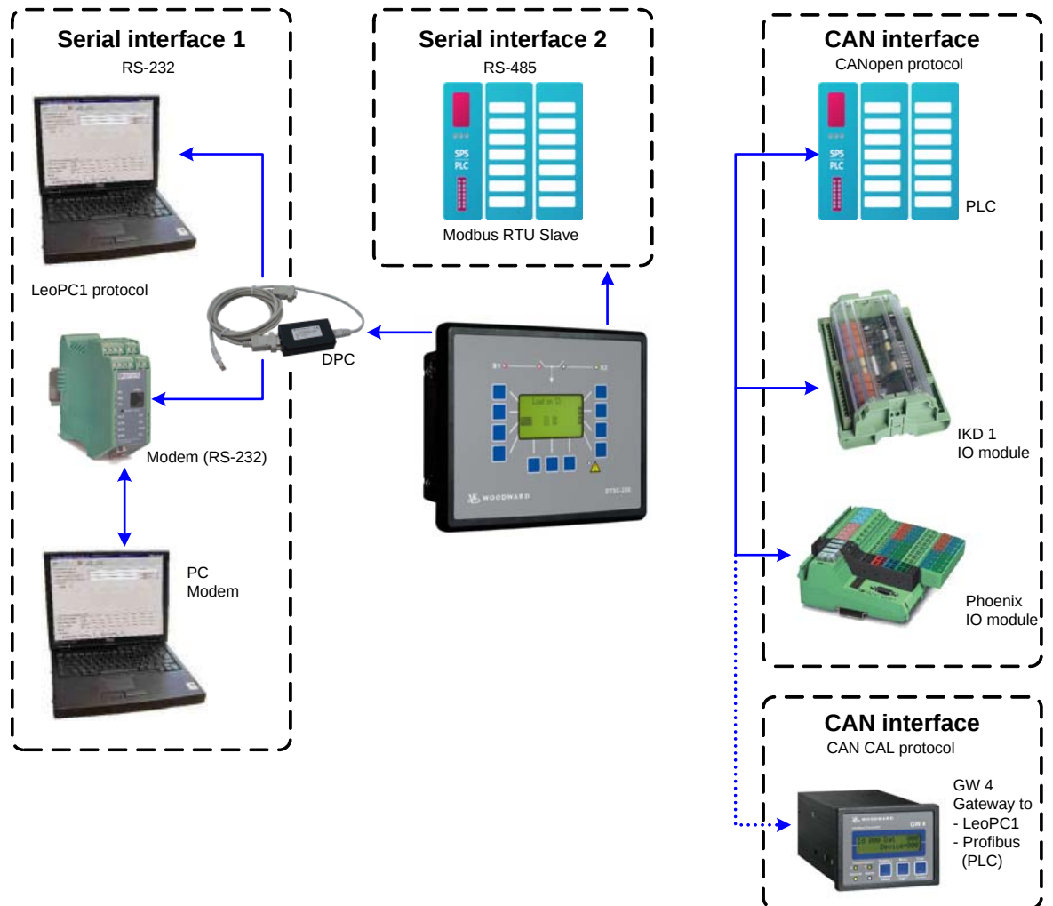
Figure 1-1: Interface overview
