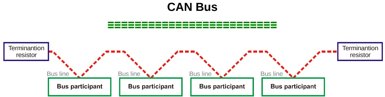
Figure 1-4: CAN bus topology
